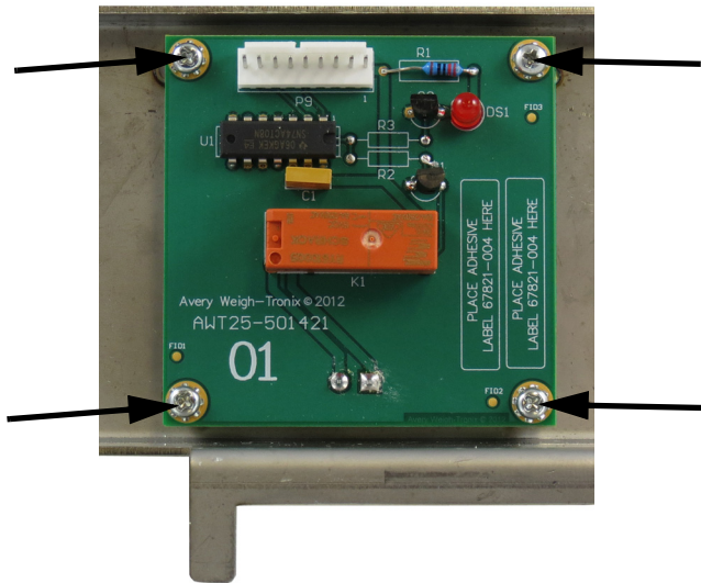
Figure 4 Relay card in place
