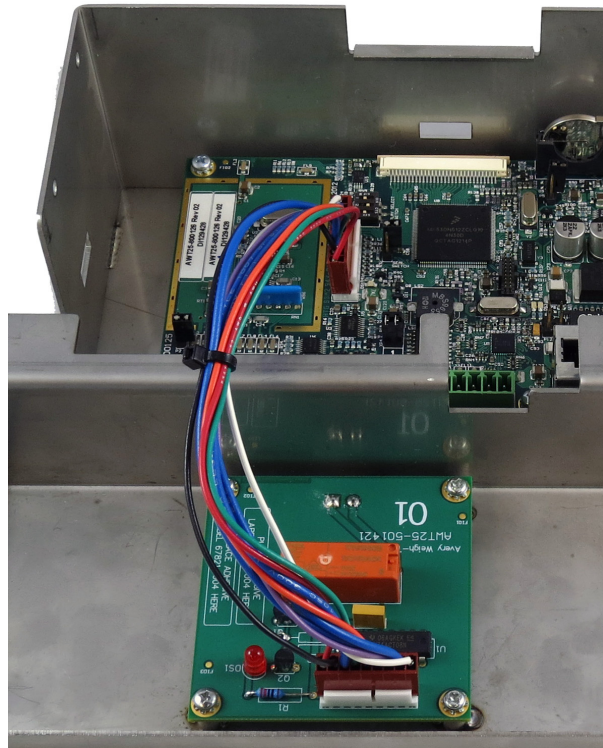
Figure 5 Cable connection
